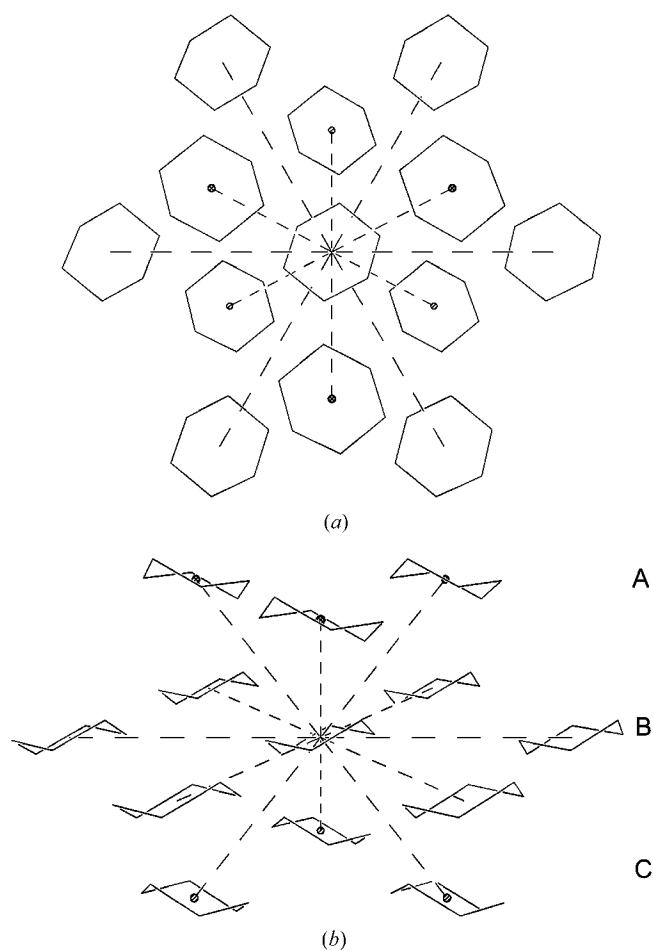
Figure 7 Molecular coordination in cyclohexane-II (CSD refcode: CYCHEX). The distribution of the molecular centroids resembles that in a cubic close-packed structure, with layers following an ...ABCABC... pattern. Layers viewed from the top (a) and side (b). Centroids in layers A and C are marked with a circle containing a cross (top layer) or a diagonal line (bottom layer), respectively. H atoms are omitted for clarity.
